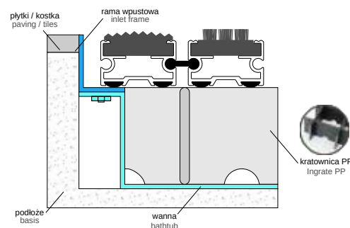
Instalacja w wannie System Plus Installation in bathtub System Plus
